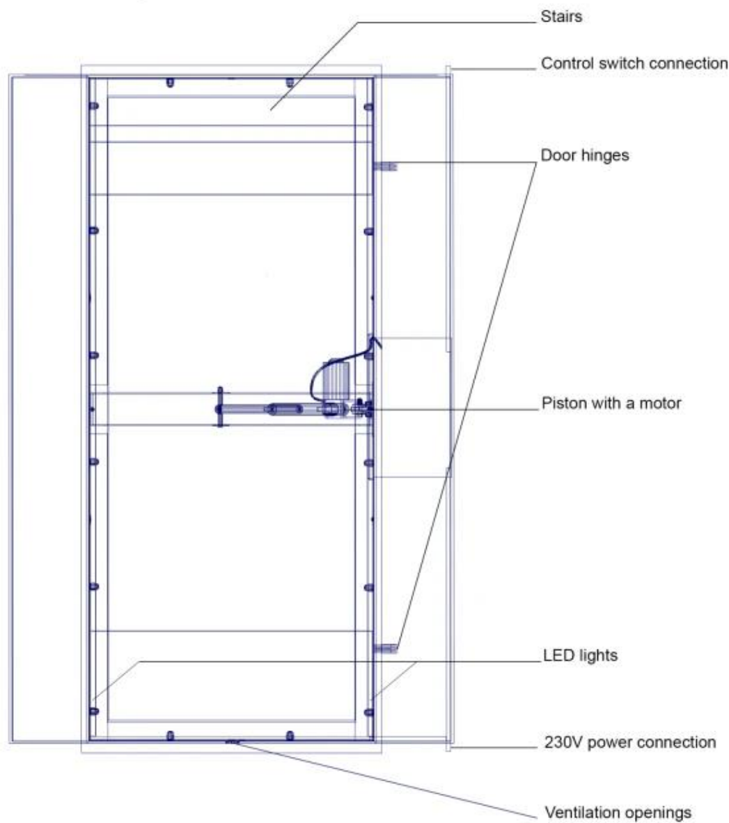
Configuration A
