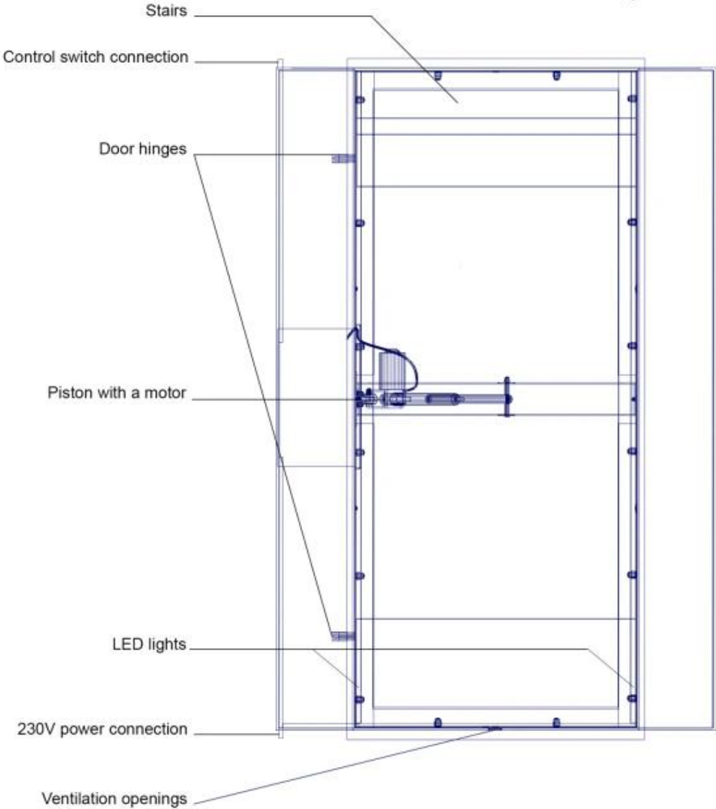
Configuration B
